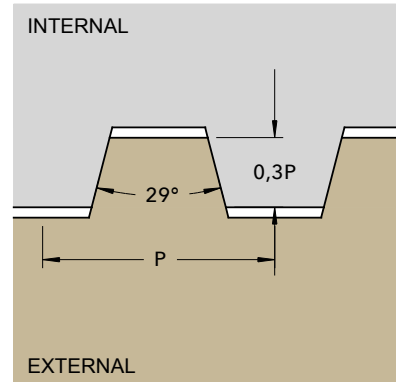
STUB ACME
