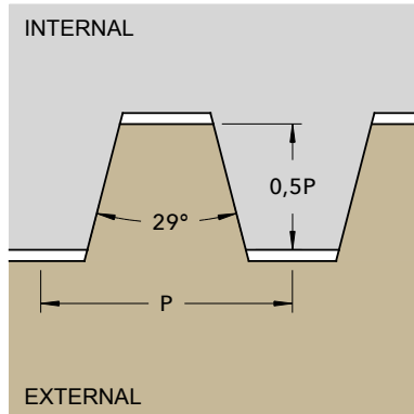
ACME
