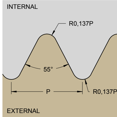
Whitworth (W)
