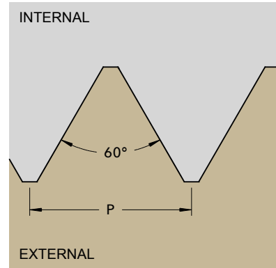
NPSF
