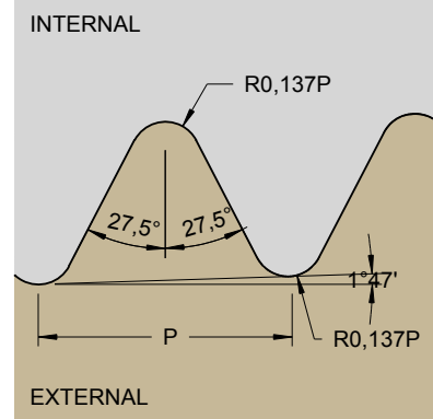
BSPT
